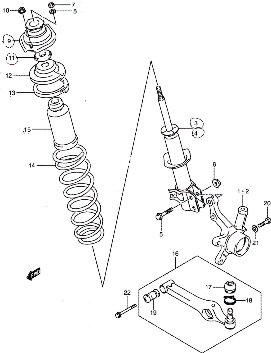
HE21S_416B FRONT SUSPENSION
